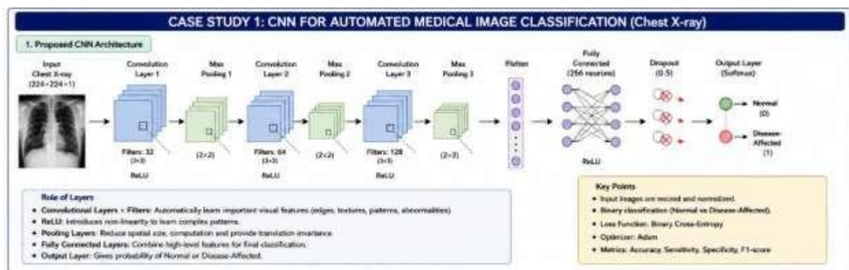
Figure 1: CNN FOR AUTOMATED MEDICAL IMAGE CLASSIFICATION
